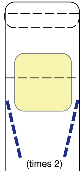
Vertical Spar Pocket (3.9 oz. Dacron) with Kevlar patch, sew closed on an angle to create a triangular opening
