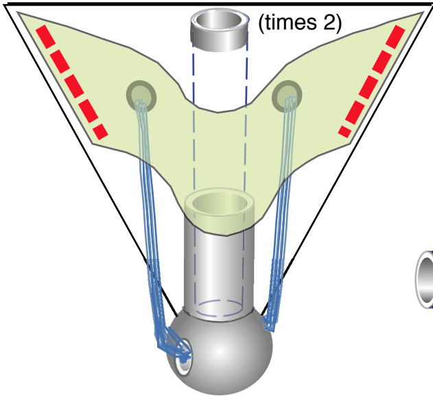
Vertical Spar Patch (3.9 oz. Dacron) with a cover sewn over the elastic & knots
